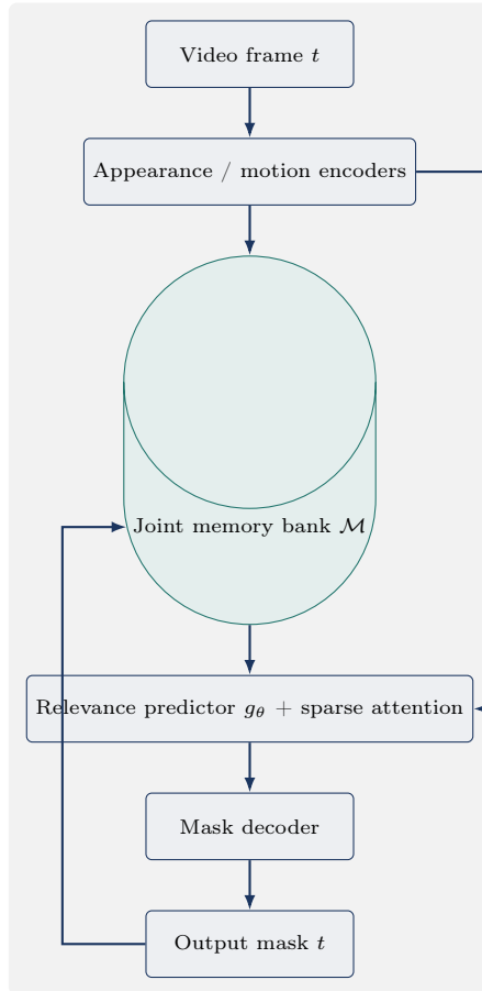
Fig. 1: SparseFlow pipeline. Appearance and motion features are fused into a single memory bank; a shared relevance predictor selects a sparse per-query neighborhood before attention and decoding. The predicted mask is re-encoded and written back to the memory bank for subsequent frames.
