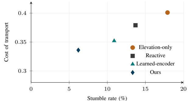
Fig. 1. Cost of transport versus stumble rate, pooled across all five terrain classes. Lower-left is better on both axes.
