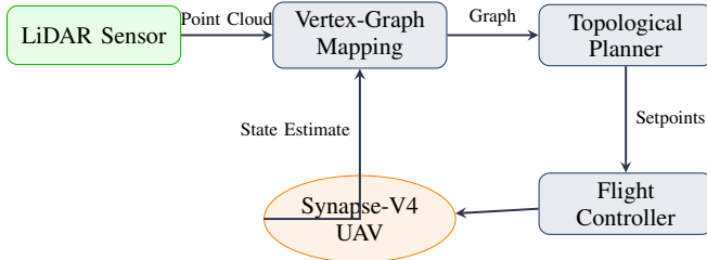
Fig. 1. System architecture of the proposed autonomous navigation framework. The Synapse-V4 platform utilizes solid-state LiDAR data to construct the Vertex-Graph, which guides the topological path planner.
