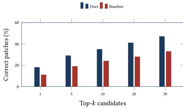
Figure 2: Correct-patch rate as a function of candidate budget k , averaged over the three benchmarks.
