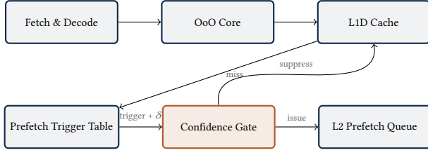
Figure 1: SpecGate sits between the L1D miss path and the L2 prefetch queue. The Confidence Gate consults the trigger table’s per-entry counter before a predicted address is allowed to issue.
