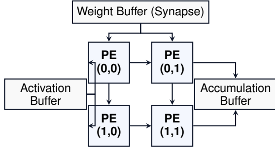
Fig. 1. Microarchitecture of the Vertex-Flow PE array with dynamic routing. Activation and weight streams are managed locally.
