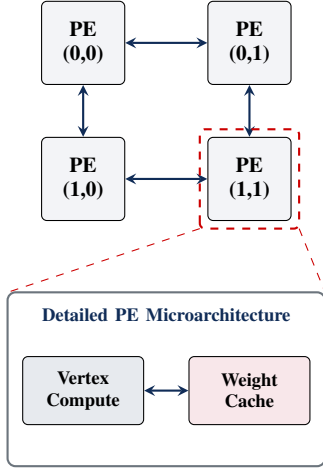
Fig. 1. Nexa 2D Mesh Multi-Core Architecture and Processing Element (PE) Microarchitecture.
