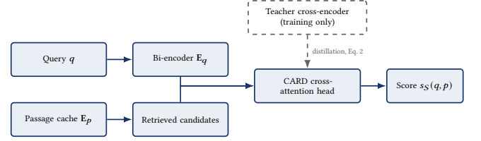
Figure 1: CARD serving-time pipeline. Query and passage embeddings are produced by a frozen bi-encoder; the passage side is pre-computed offline. Only the lightweight cross-attention head runs per candidate at query time. The cross-encoder teacher (dashed) supervises the head during training and is never invoked at serving time.
