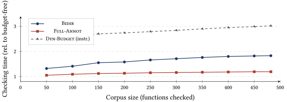
Fig. 1. Checking-time overhead relative to a budget-free typechecker, as corpus size grows. BIDIR tracks close to FULL-ANNOT despite inferring most cost bounds; the instrumented DYN-BUDGET baseline is shown for reference only, since its cost is a run-time overhead rather than a checking-time one.
