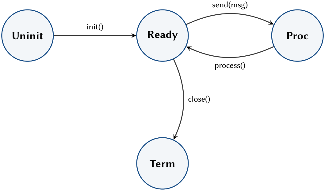
Fig. 1. The lifecycle state machine of an actor protocol in Synapse. Edges represent transition-triggering actions.
