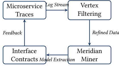
Fig. 1. Architectural overview of the proposed Meridian-Spec framework. The system processes raw microservice traces via Vertex Filtering, executes contract mining, and generates formal interface specifications.
