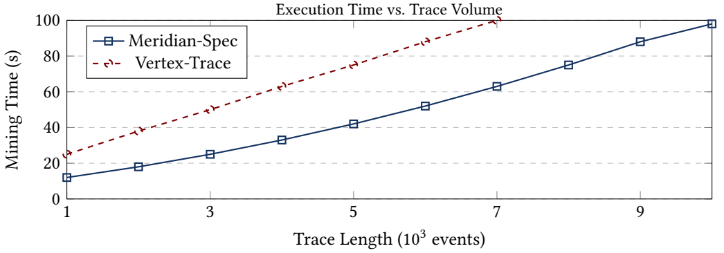
Fig. 2. Comparison of mining overhead between Meridian-Spec and Vertex-Trace as a function of request trace length.
