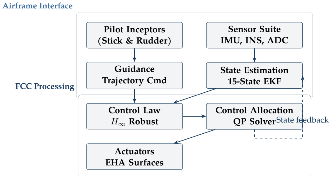
Figure 2.1: AFCS functional architecture — data flow and processing layers.
