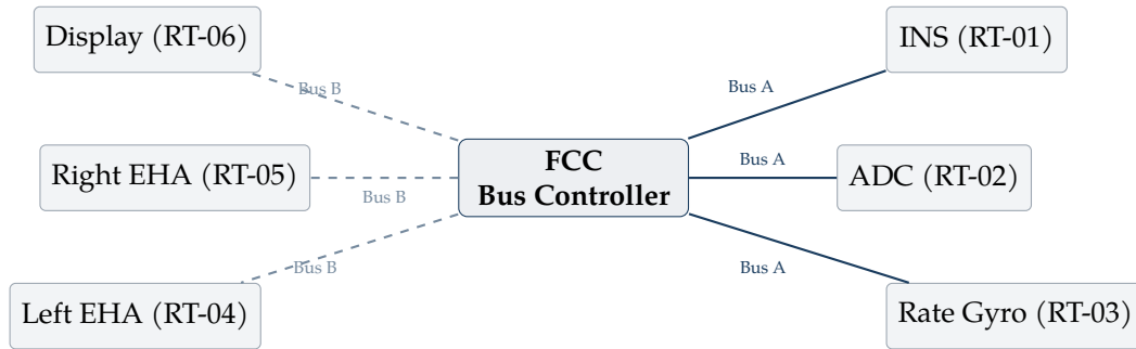
Figure 2.2: Dual-redundant MIL-STD-1553B bus topology. Solid lines = Bus A; dashed lines = Bus B.
